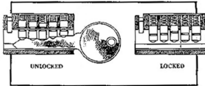
Figure 8. A pin tumbler lock.
