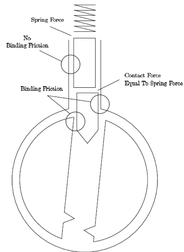
Figure 5.4: Key pin enters hull
