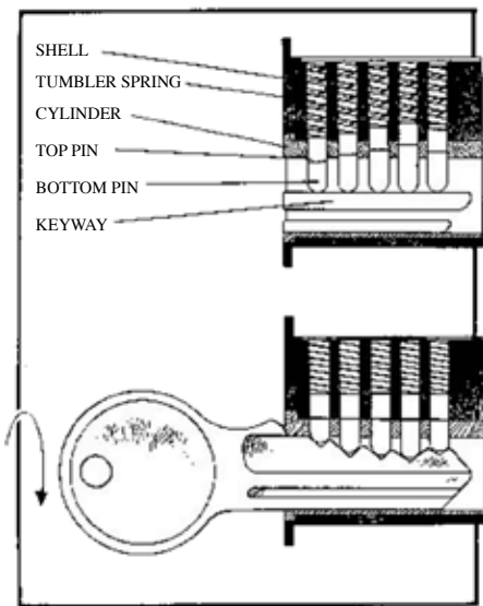
Figure 1. The pin tumbler lock, cutaway view.
