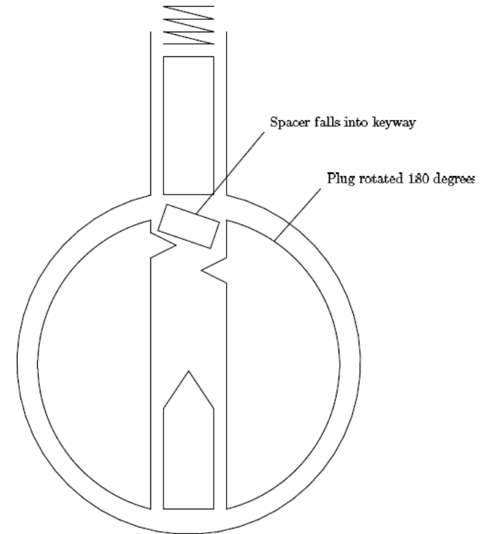
Figure 9.9: Spacer or driver can enter keyway
