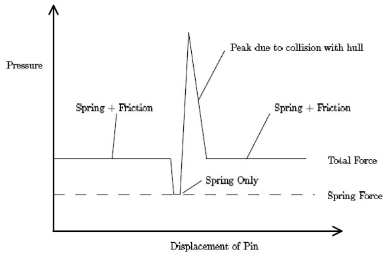
Figure 5.5: Pressure required to move pins
