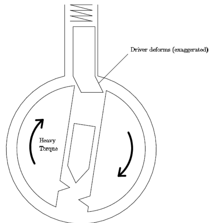
Figure 9.2: Driver pin false set by elastic deformation
