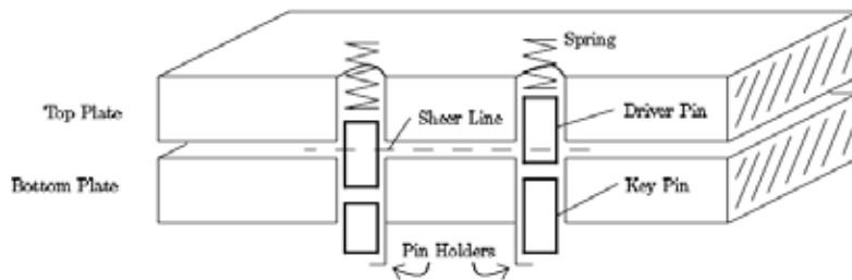
Figure 3.1: Flatland model of a lock
