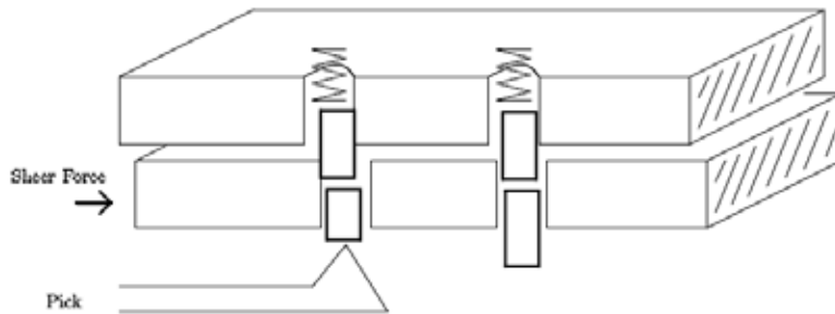
Figure 4.2: (b) Pick lifts the binding pin
